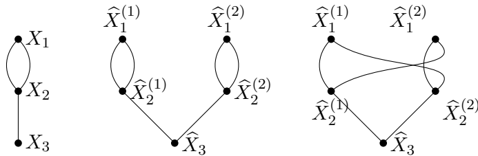
FIGURE 2. The level graphs \bar{\Gamma} , \widehat{\Gamma}_1 , and \widehat{\Gamma}_2
