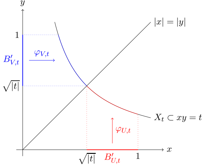
Figure 2: The maps \varphi_{U,t} and \varphi_{V,t} .
